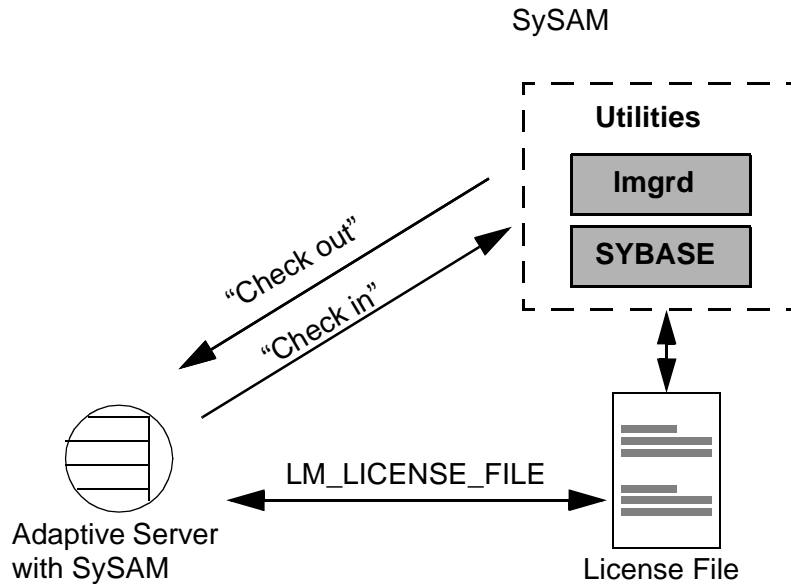
Figure 4-1: SySAM Components
