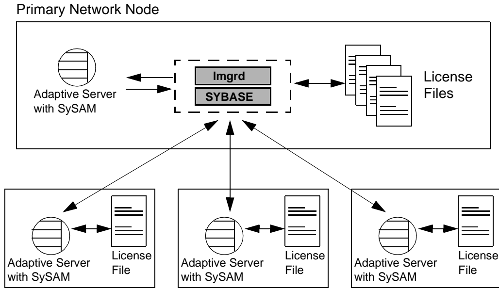
Figure 4-3: Network system
